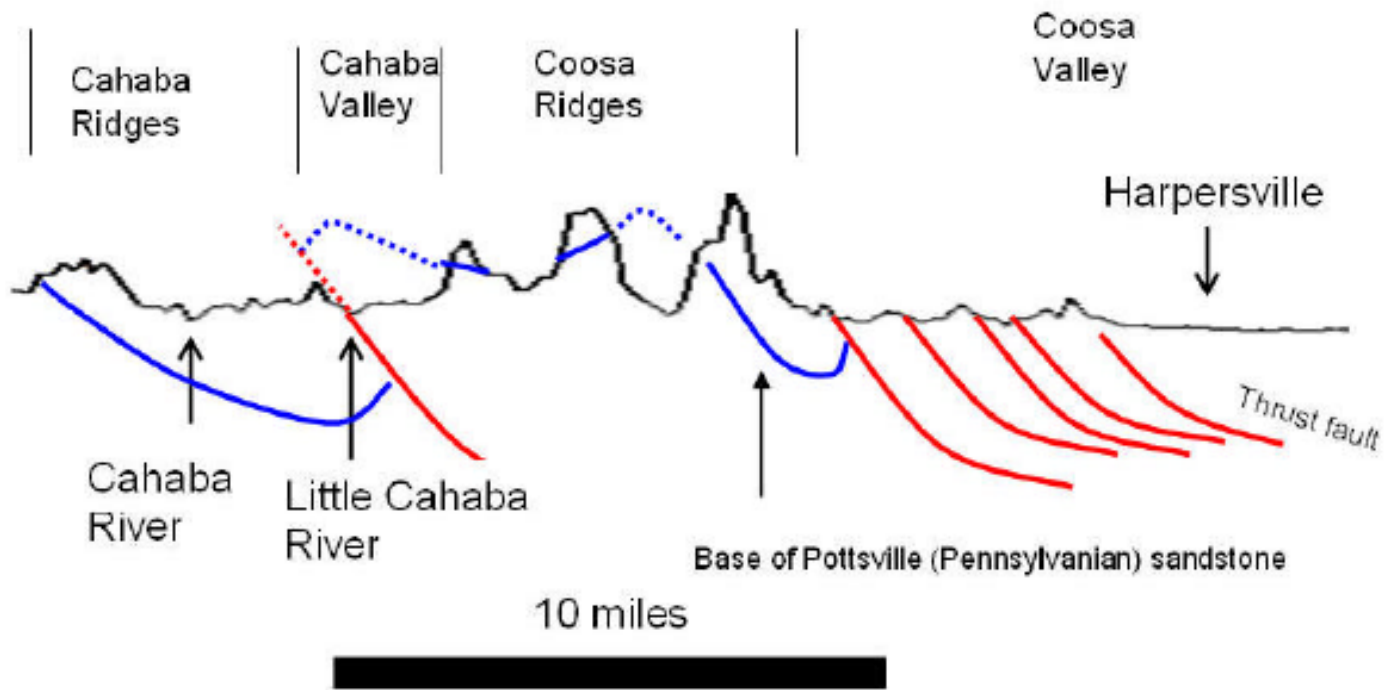
Figure 4. NW-SE topographic profile showing most of the physiographic districts in the Valley and Ridge and their relationship to the underlying geology. Relief and dip of rocks are exaggerated. Red lines: thrust faults, blue line: base of the Pottsville sandstone (Location 2 on Figure 1).
