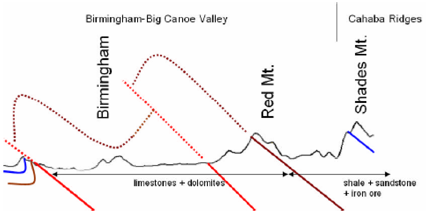
Figure 3. NW-SE topographic profile through Birmingham showing the location of the Red Mountain Formation (brown), major thrust faults (red), and base of the Pottsville sandstone (blue). The dotted lines show the approximate locations of the rocks and the faults before erosion (Location 1 on Figure 1).
