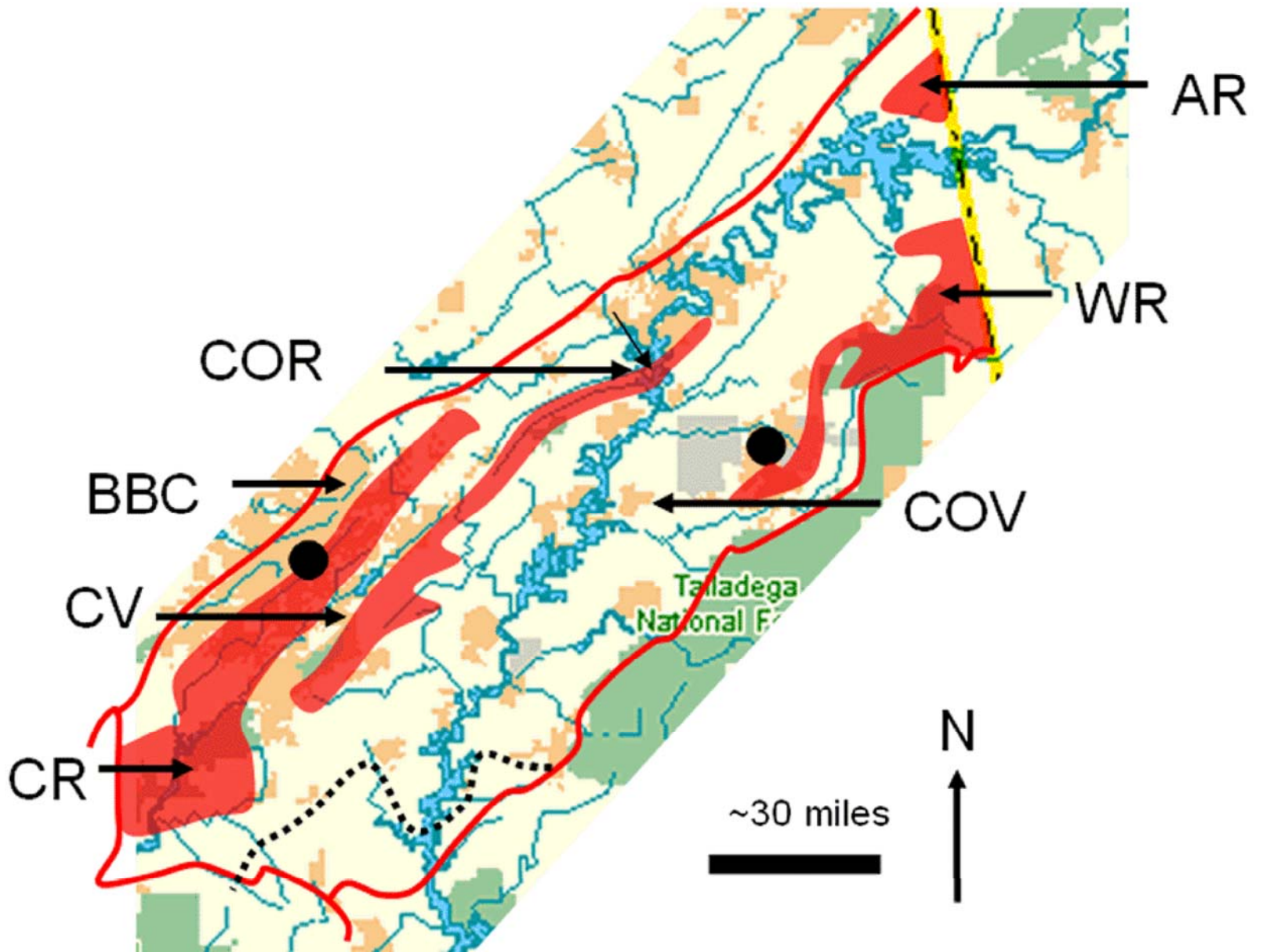
Figure 2. Physiographic districts of the Valley and Ridge. AR: Armuchee Ridges, BBC: Birmingham-Big Canoe Valley, CV: Cahaba Valley, CR: Cahaba Ridges, COV: Coosa Valley, COR: Coosa Ridges, WR: Weisner Ridges. Red lines: boundaries of the Valley and Ridge, red-filled areas: ridge districts. Black Circles west to east: Birmingham, Anniston (USGS National Map Viewer and Geological Survey of Alabama)
