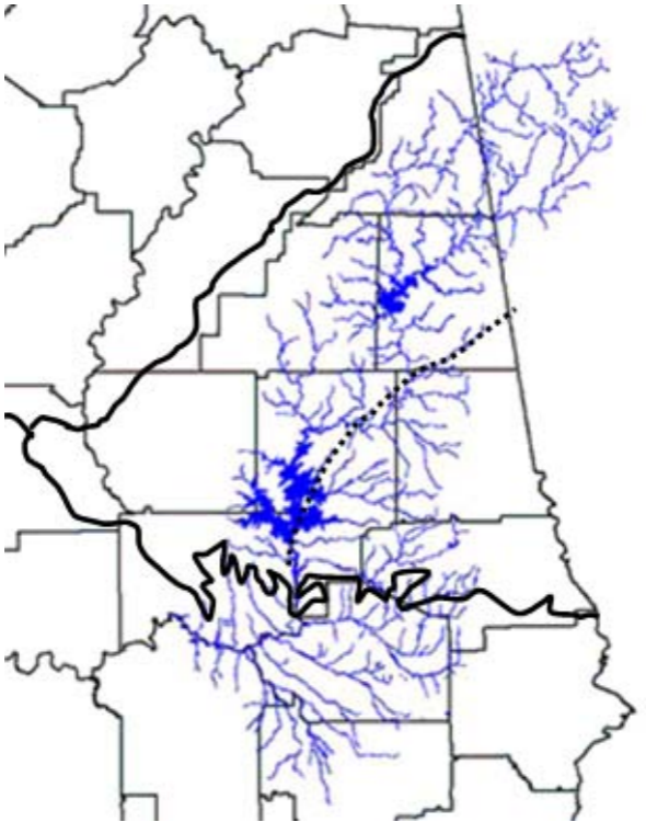
Figure 3. Drainage pattern of the Tallapoosa River and its tributaries. (Pattern from Alabama Water Watch)
