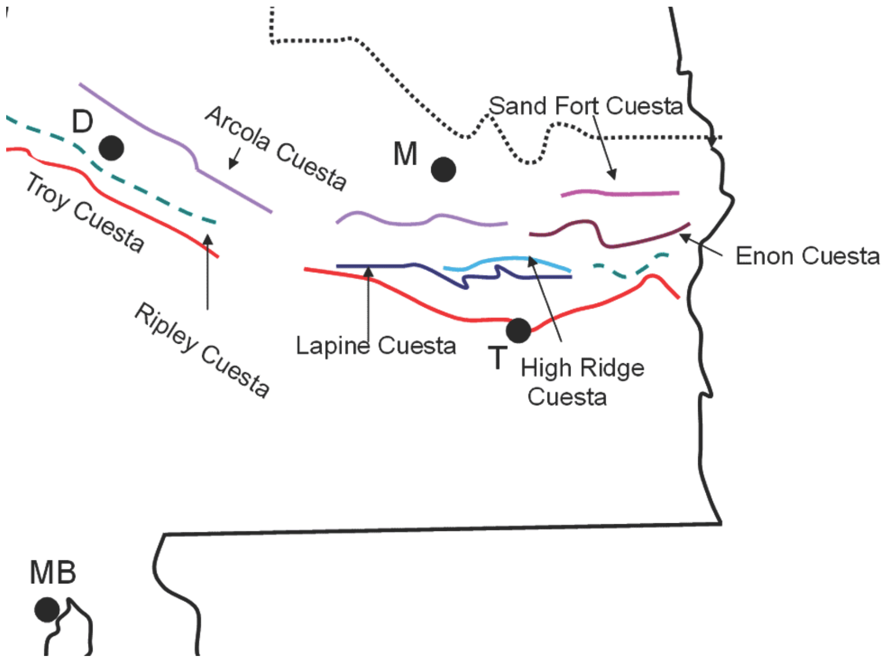
Figure 3. Locations of the major cuestas in the Coastal Plain. Broken black line: northern boundary of the Coastal Plain. Black circles: D: Demopolis, M: Montgomery, MB: Mobile, T: Troy. Cuesta names from Sapp and Emplaincourt 1975
