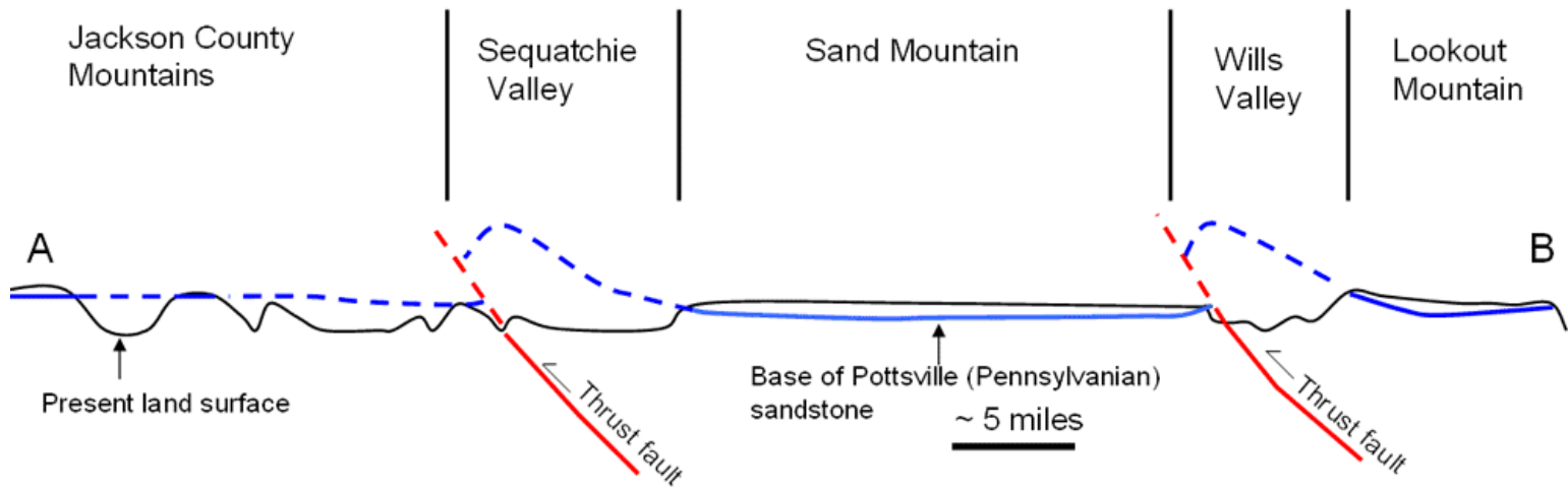
Figure 3: Cross-section A-B (see Figure 1 for location) showing the major geologic structures in the Cumberland Plateau. The blue line shows the base of the Pottsville Formation, the most resistant rock in the area. The blue and red broken lines show the approximate location of the Pottsville and the thrust faults before erosion has reduced the surface to the black solid line.
